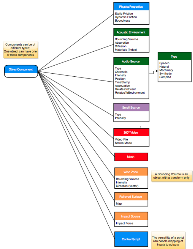
Figura 3 - Object Component e Script Component.
